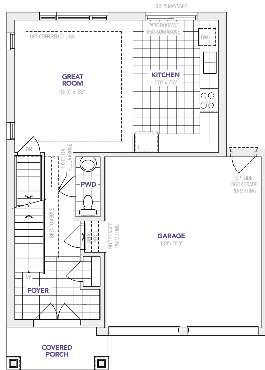
ELEVATION A MAIN FLOOR
