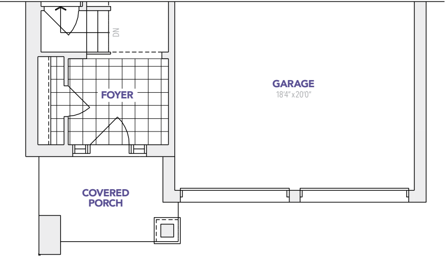
B PARTIAL MAIN FLOOR
