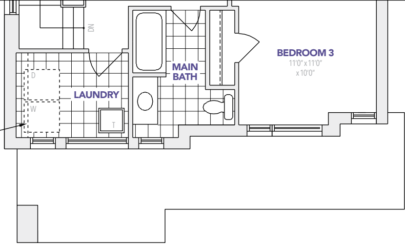
B PARTIAL SECOND FLOOR
