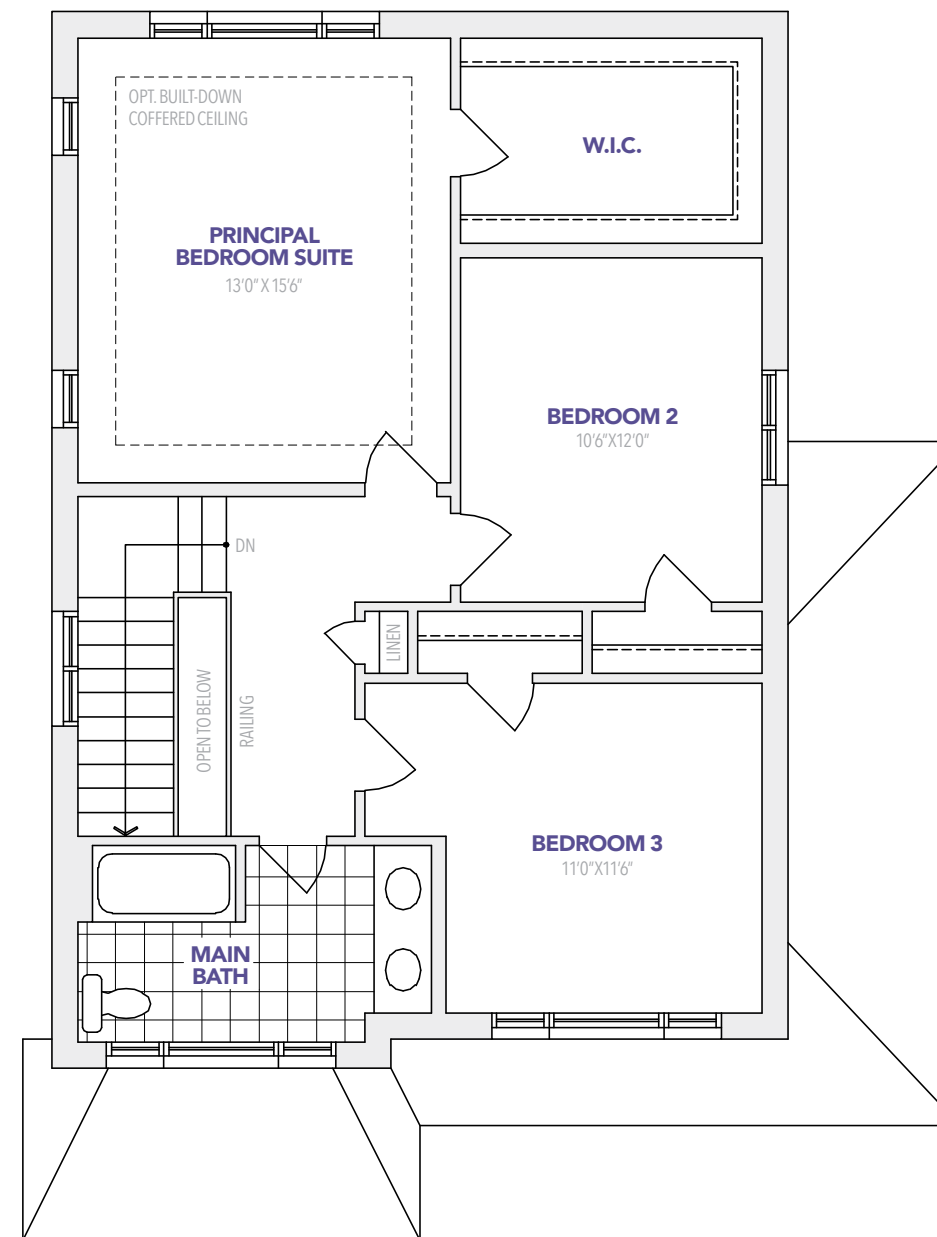
ELEVATION A SECOND FLOOR
