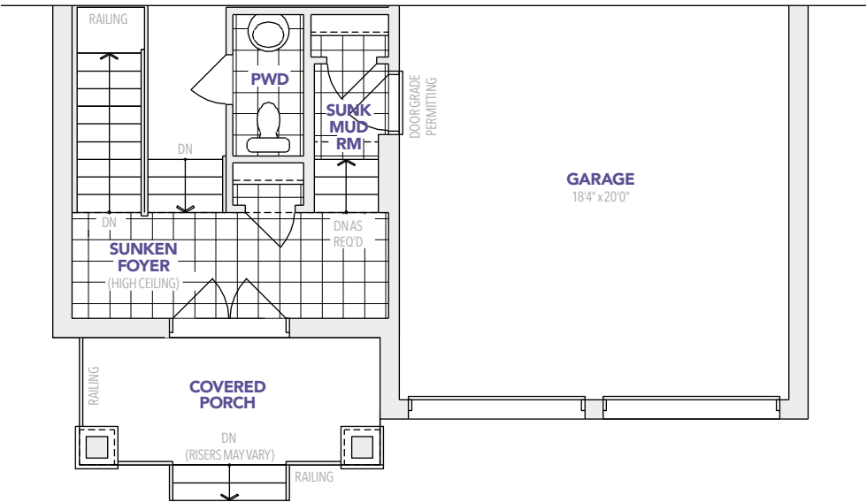
B PARTIAL MAIN FLOOR
