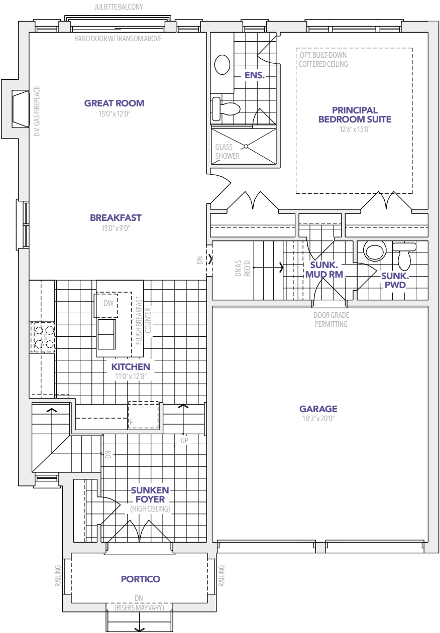
A MAIN FLOOR
