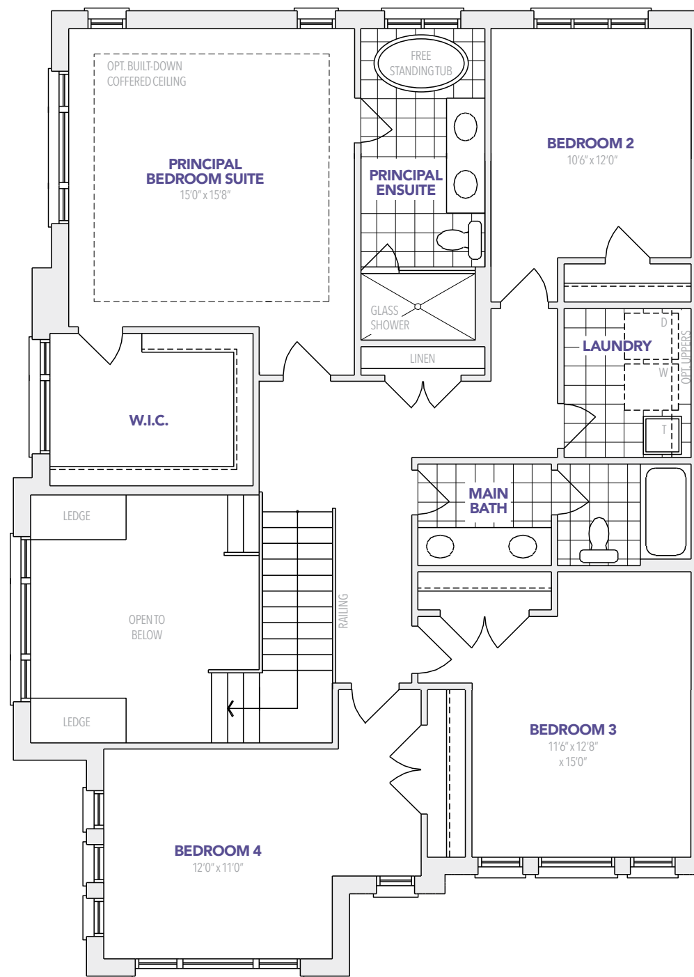
ELEVATION B SECOND FLOOR
