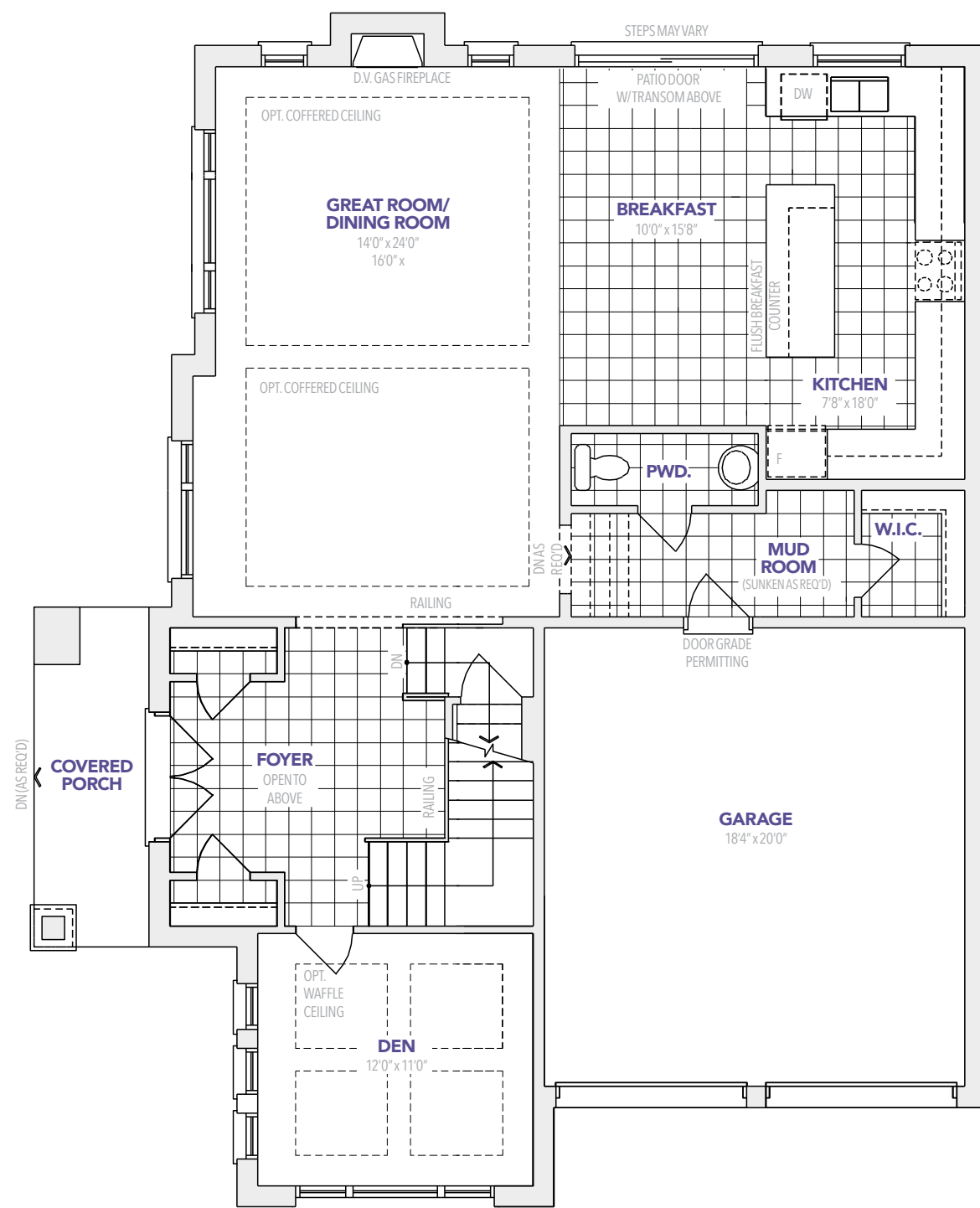
ELEVATION B MAIN FLOOR
