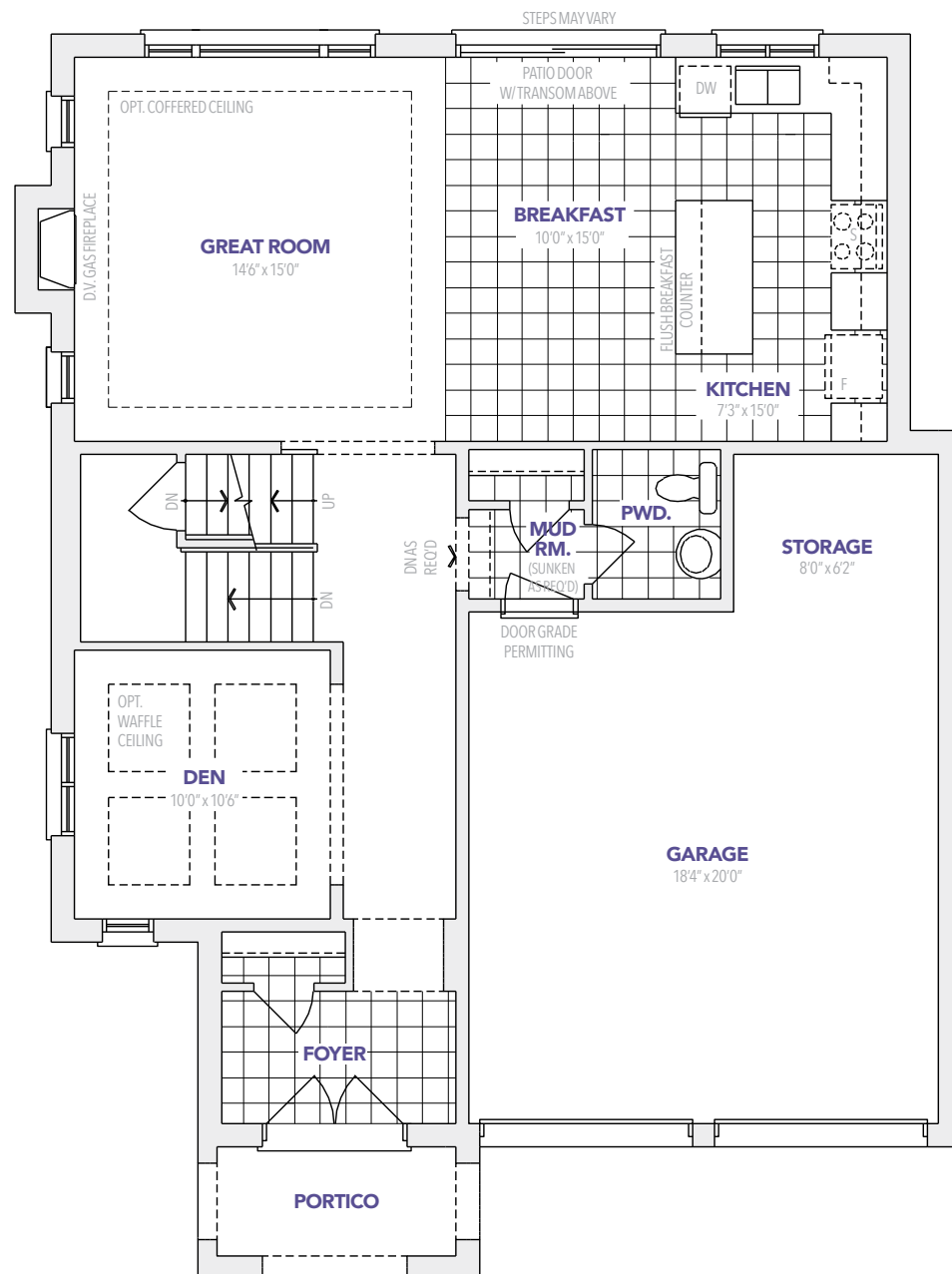
ELEVATION A MAIN FLOOR
