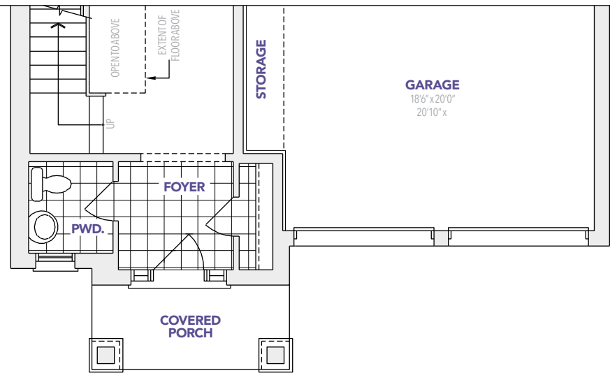
B PARTIAL MAIN FLOOR
