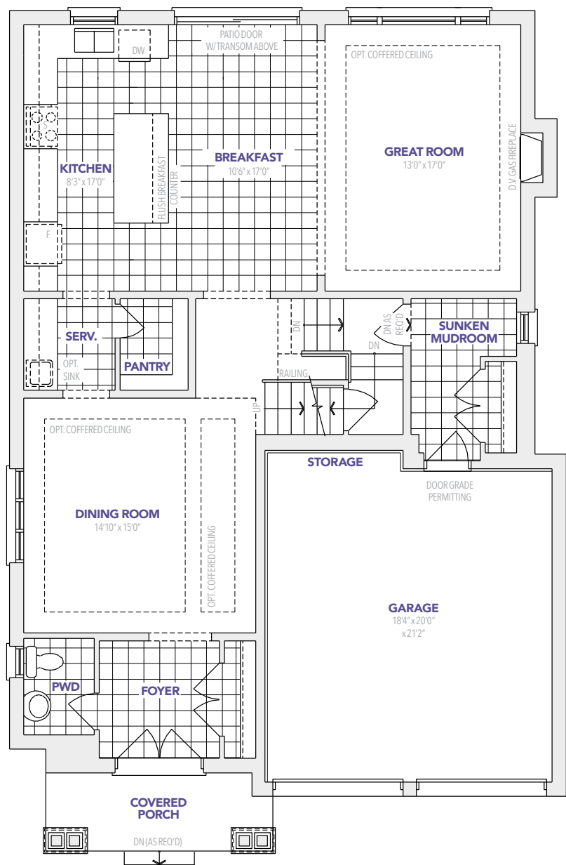
A MAIN FLOOR
