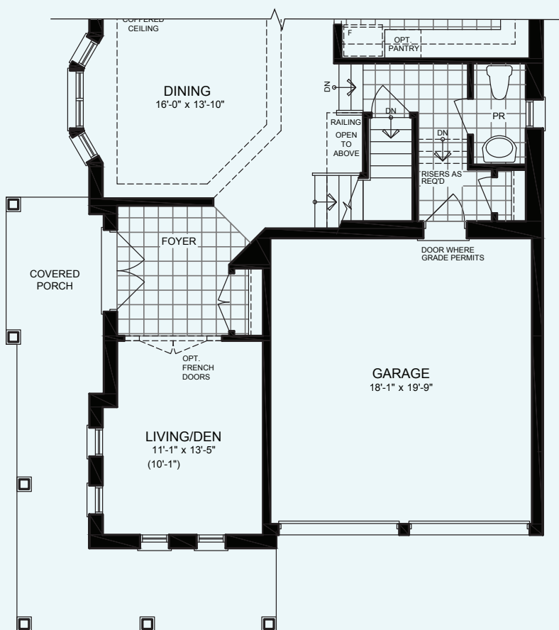
PARTIAL GROUND FLOOR PLAN ELEVATION B
