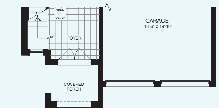
PARTIAL GROUND FLOOR PLAN ELEVATION B
