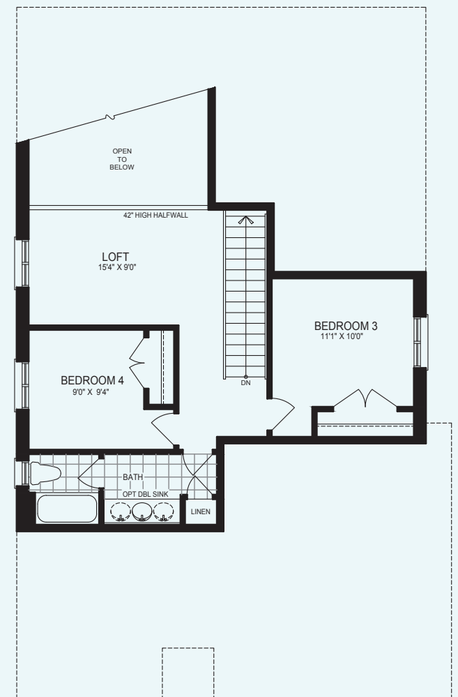
LOFT PLAN ELEVATION B
