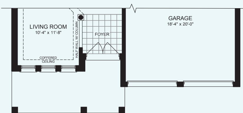
PARTIAL GROUND FLOOR PLAN ELEVATION B
