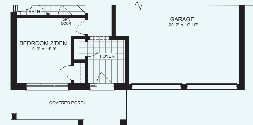
PARTIAL GROUND FLOOR PLAN ELEVATION B
