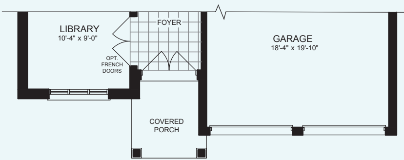
PARTIAL GROUND FLOOR PLAN ELEVATION B
